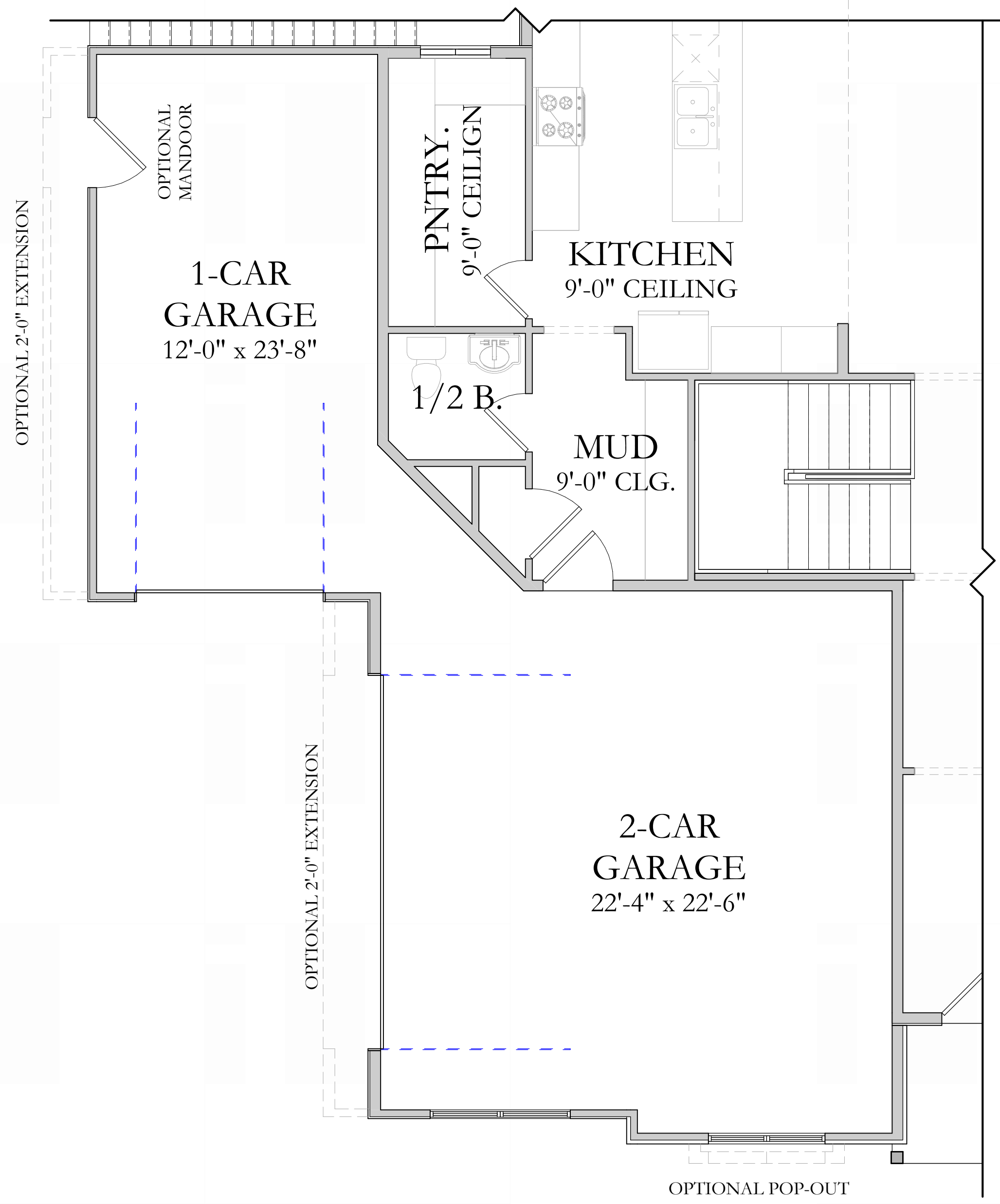
OPTIONAL SIDE LOAD 3-CAR GARAGE
